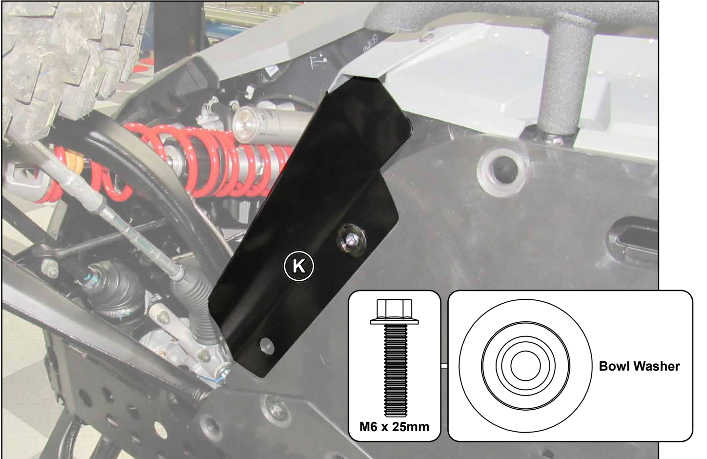
- Install Left Splash Plate (K) to stock mounting locations with hardware shown.
