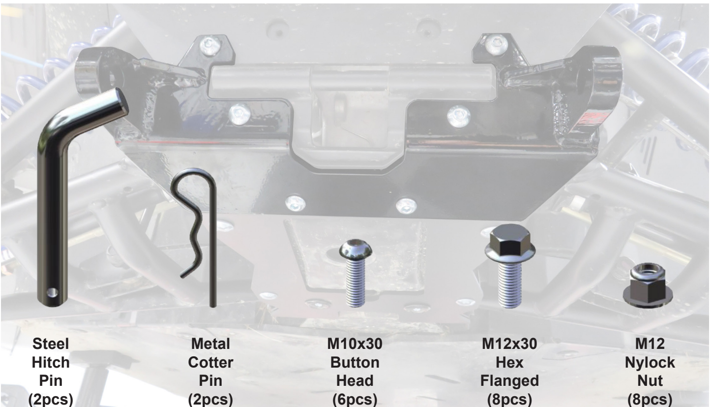
Spacer Plate
