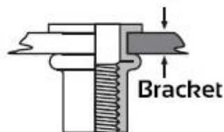
Visual Representation Of When Well Nut When Screw Tightened
