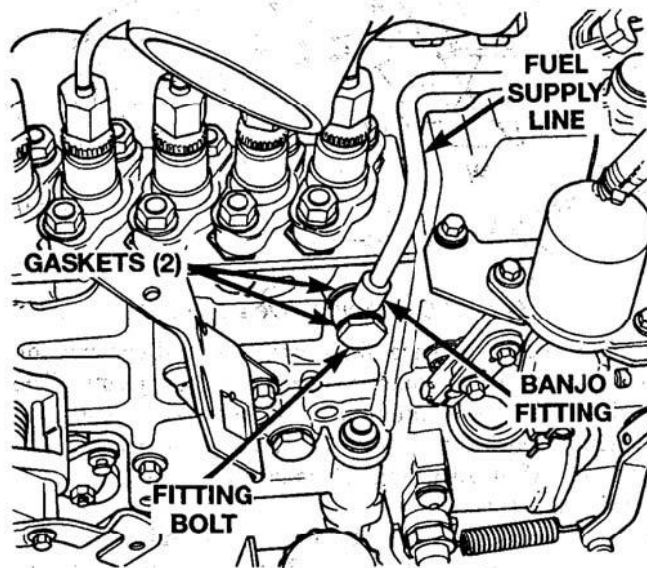
Fuel Inlet Line at Injection Pump
