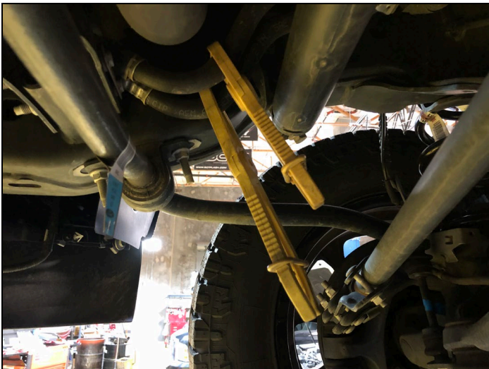
FIGURE 24 : Hose Crimp Pliers on Trans Cooler Lines
