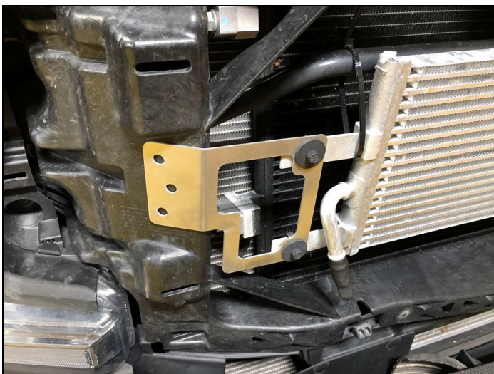
FIGURES 20 & 21 : Positioning The Cooler Using Cable Ties
