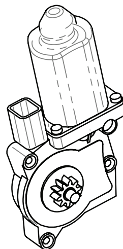
(26) x2 Motor
