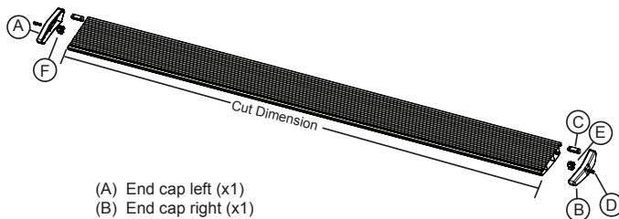
1 x2 Running board assembly
