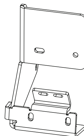
36 Linkage Mounting Bracket Driver ( Front )
